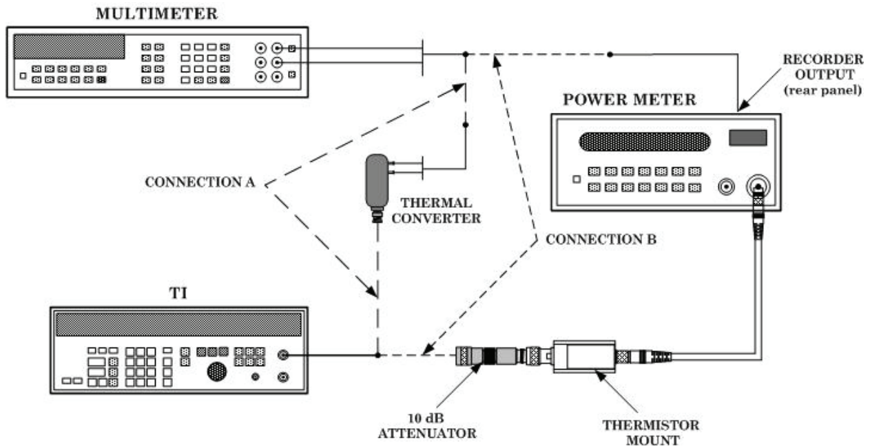
Figure 4. Flatness.
