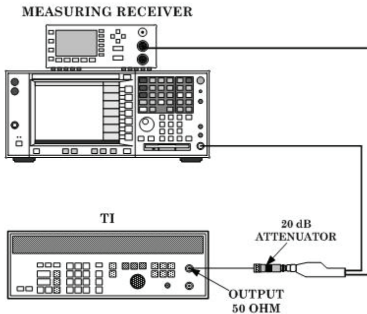
Figure 5. Attenuator accuracy.
