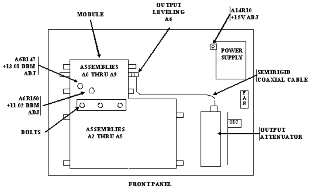
Figure 1. Test Instrument – top view.
