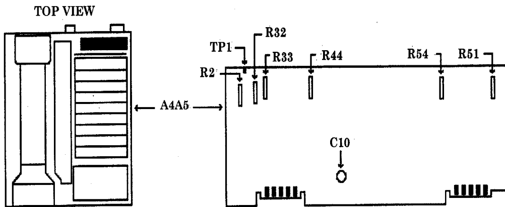
Figure 15. A4A5 board.
