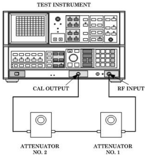
Figure 16. Attenuator connection.
