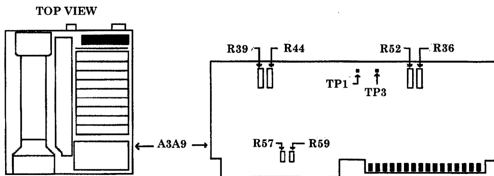
Figure 22. A3A9 board.
