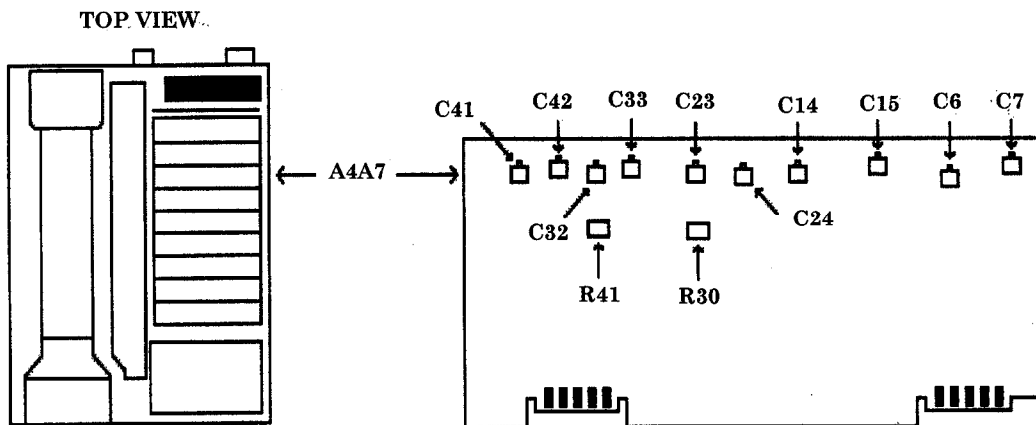
Figure 12. A4A7 board view 1.
