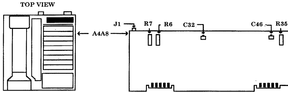
Figure 13. A4A8 board.
